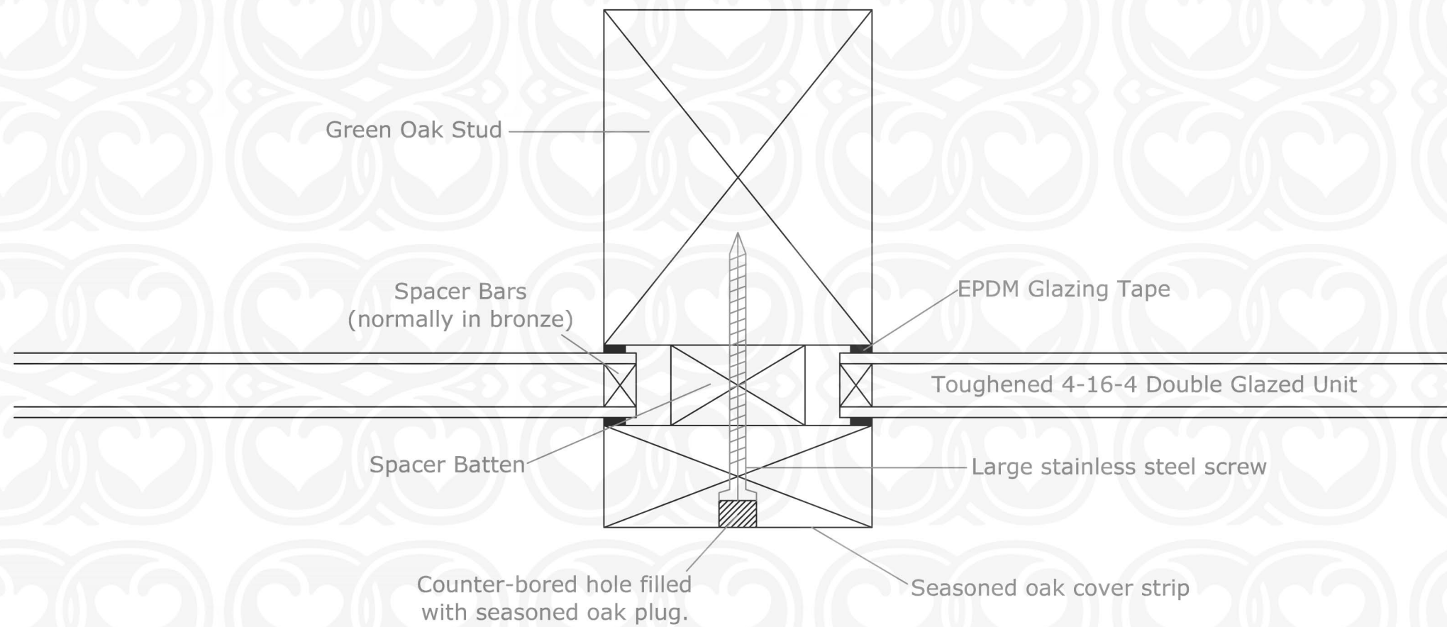
Section Through Glazing Stud
